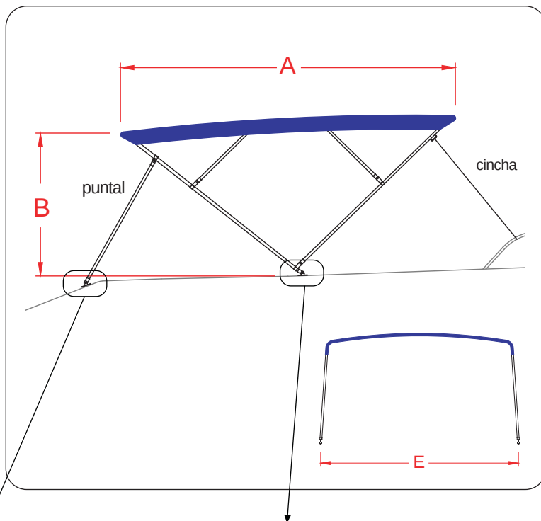
BASE BIMINI
